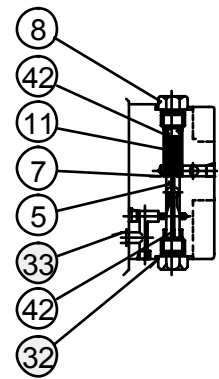
Section Q-Q
